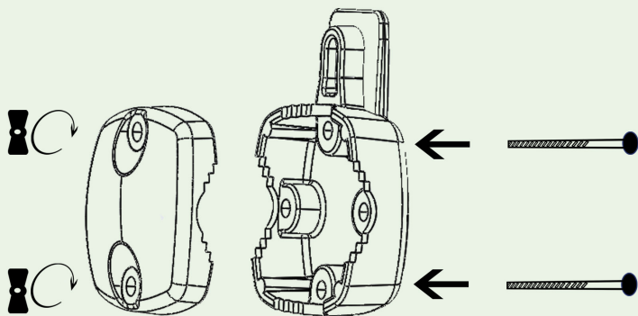
Hanger Assembly
